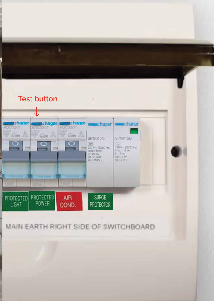
Safety Protected Switchboard
